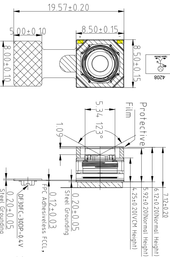
TOP VIEW
